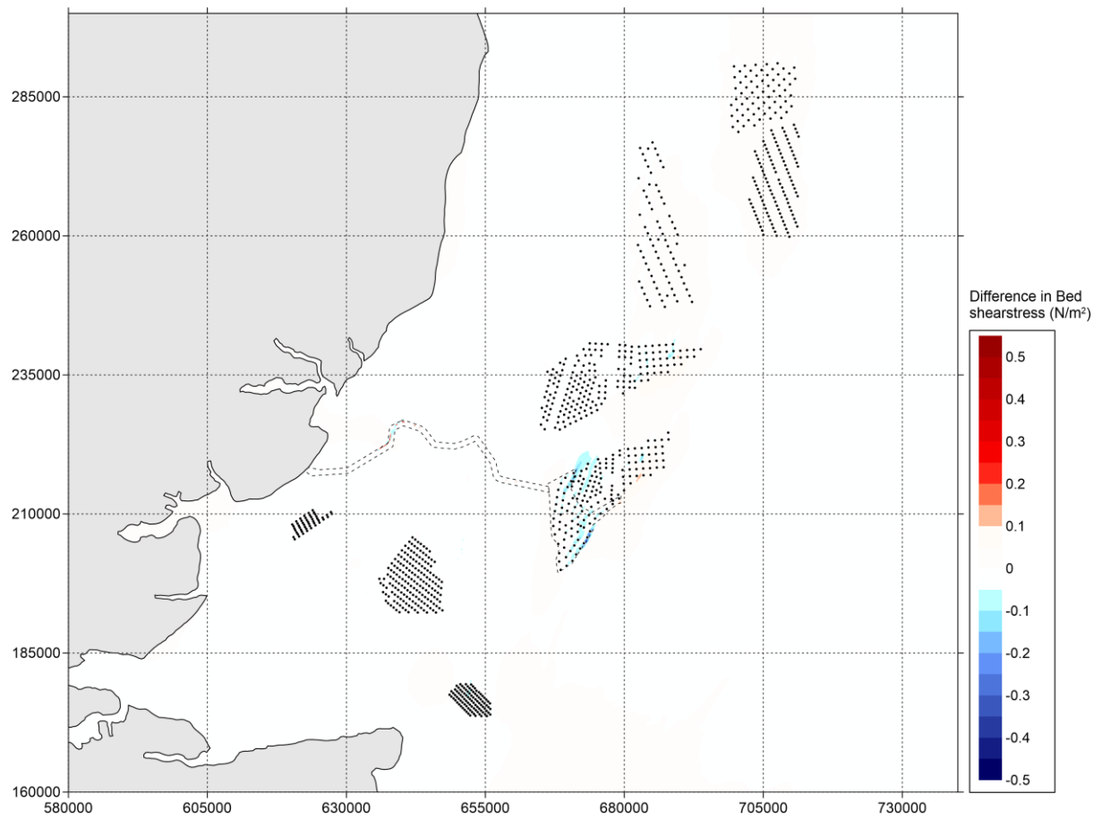
Figure 5-77 Difference in bed shear stress (in \text{N/m}^2 ) between 'Baseline' and 'Cumulative' during spring tide (positive means increase of bed shear stress by option and vice versa) – peak ebb
