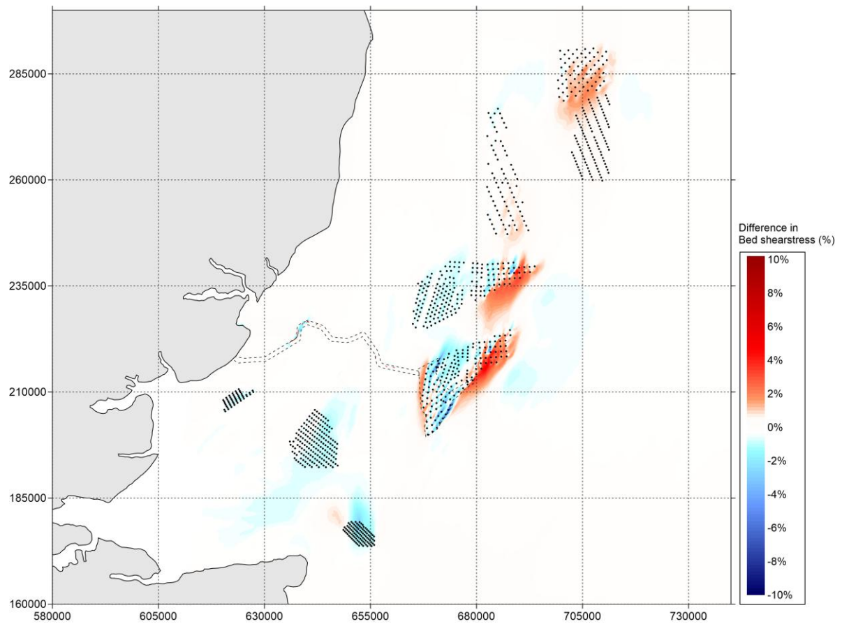
Figure 5-79 Difference in bed shear stress (in percent) between 'Baseline' and 'Cumulative' during spring tide (positive means increase of bed shear stress by option and vice versa) – peak ebb.
