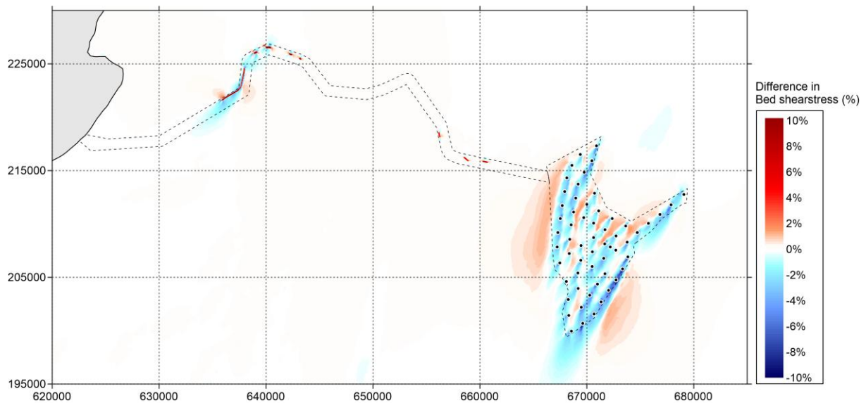
Figure 5-62 Difference in bed shear stress (in percent) between 'Baseline' and 'Option' during spring tide (positive means increase of bed shear stress by option and vice versa) – peak flood
