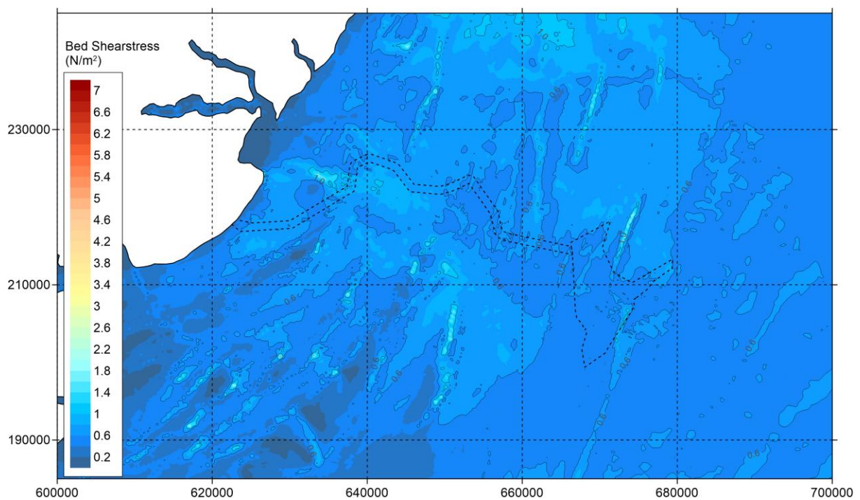
Figure 5-40 Baseline – Bed shear stress during neap tide - peak flood (zoomed in).
