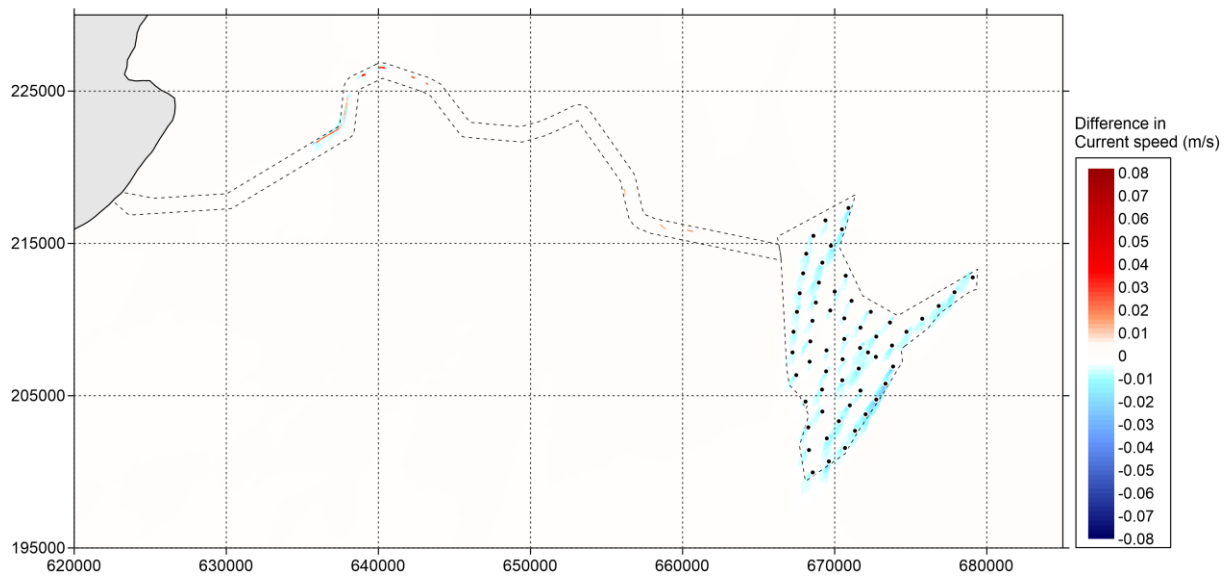
Figure 5-56 Difference in current speed (in metres/second) between 'Baseline' and 'Option' during neap tide (positive means increase of current speed by option and vice versa) – peak flood
