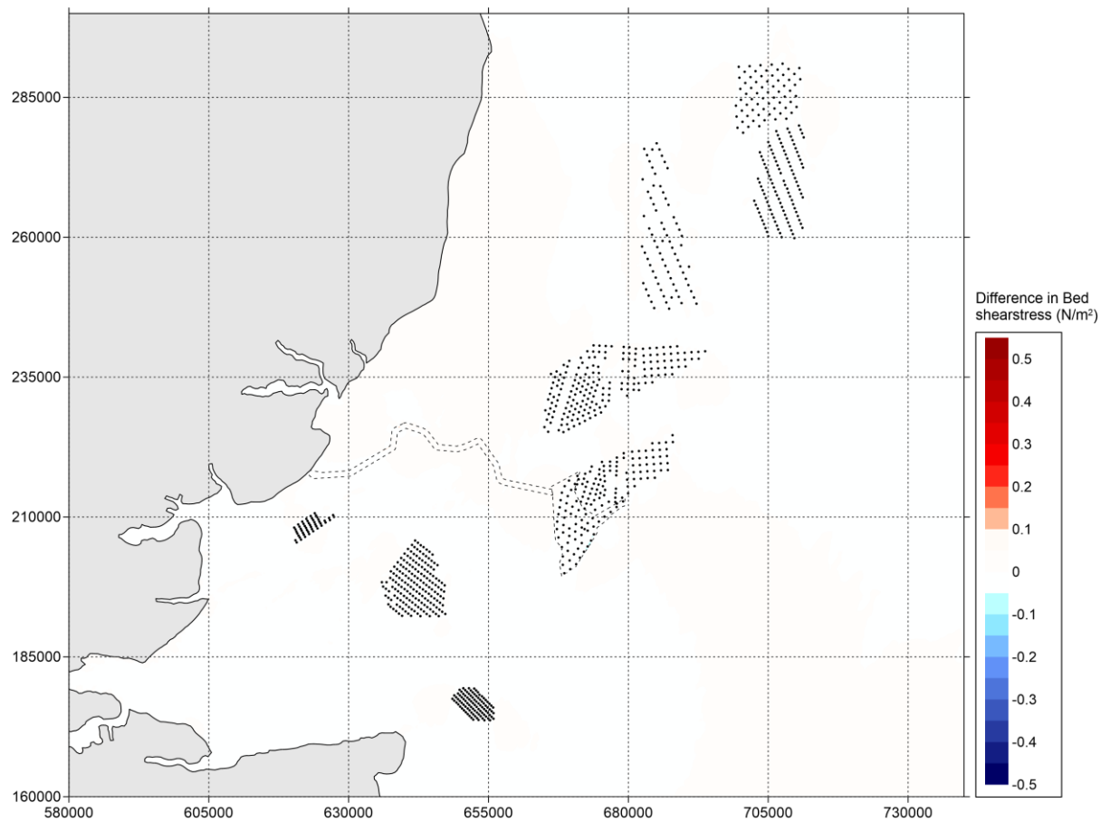
Figure 5-80 Difference in bed shear stress (in \text{N/m}^2 ) between 'Baseline' and 'Cumulative' during neap tide (positive means increase of bed shear stress by option and vice versa) – peak flood.
