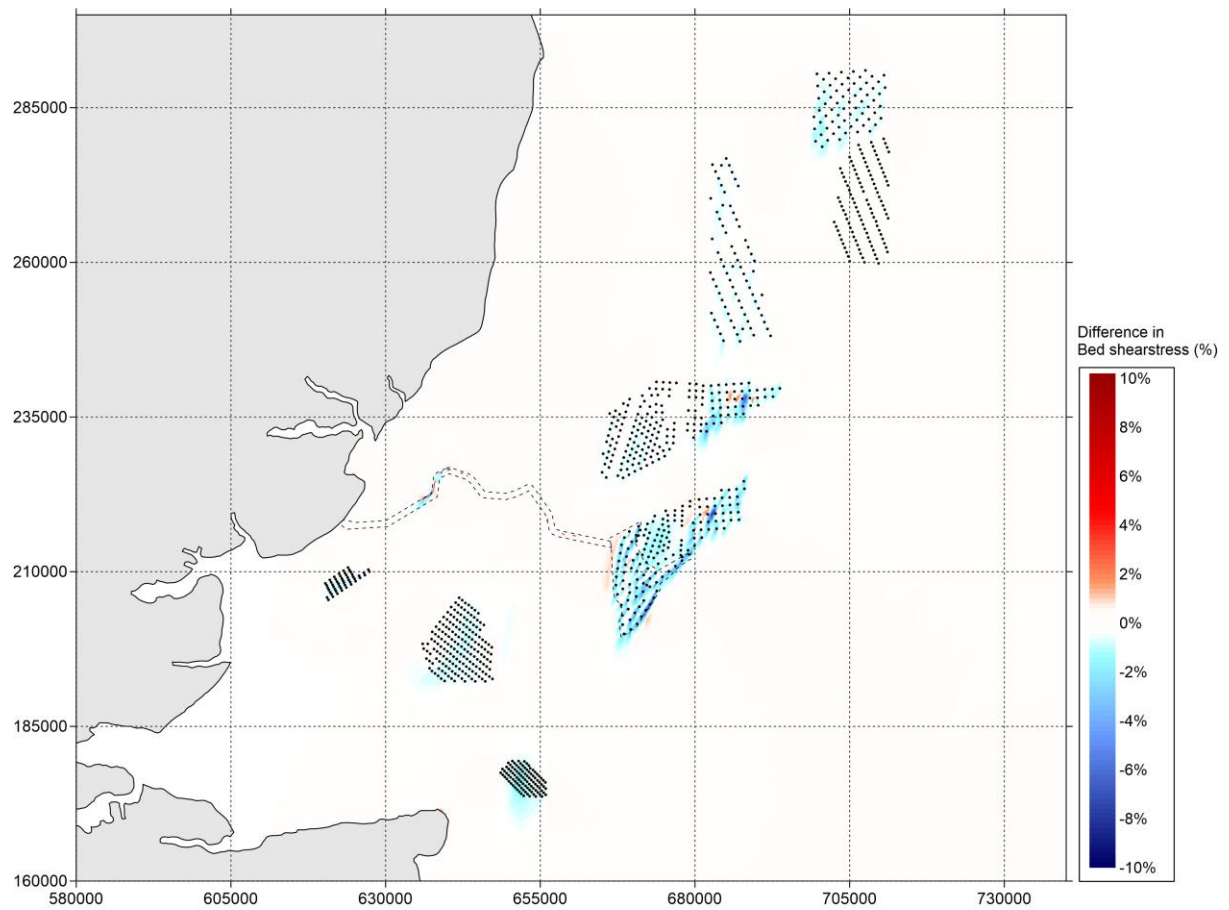
Figure 5-82 Difference in bed shear stress (in percent) between 'Baseline' and 'Cumulative' during neap tide (positive means increase of bed shear stress by option and vice versa) – peak flood.
