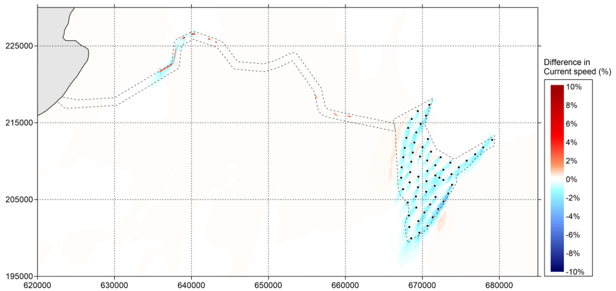
Figure 5-58 Difference in current speed (in percent) between 'Baseline' and 'Option' during neap tide (positive means increase of current speed by option and vice versa) – peak flood
