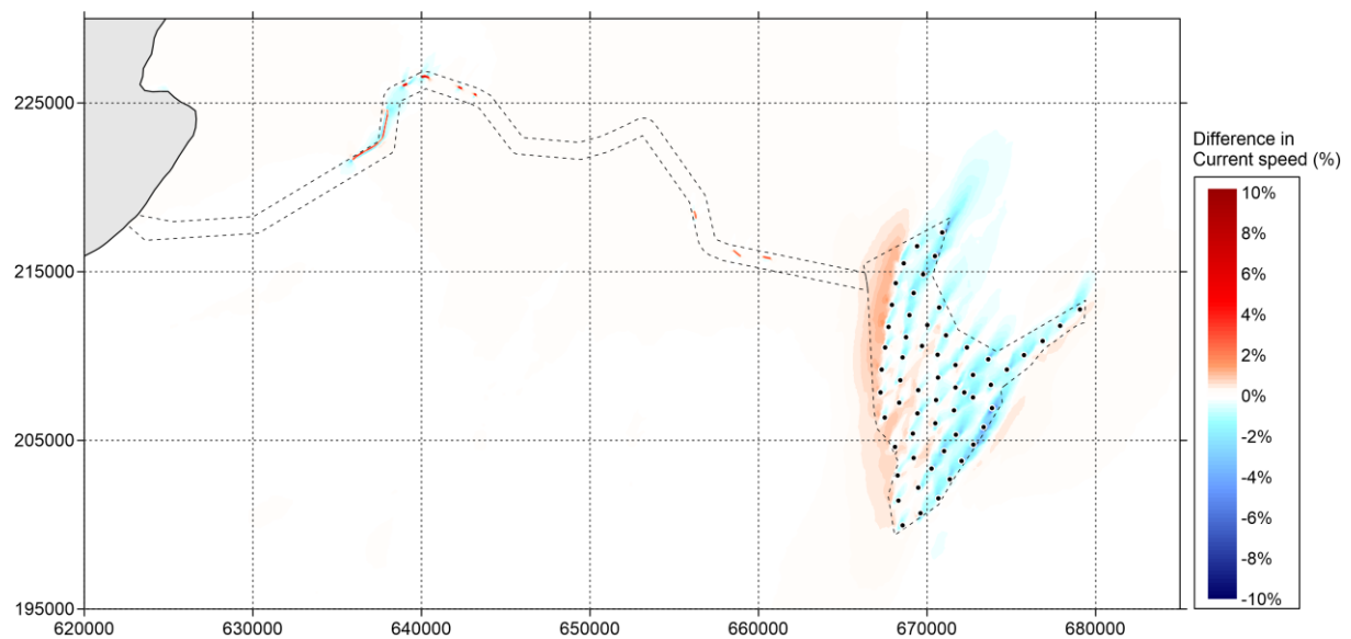
Figure 5-55 Difference in current speed (in percent) between 'Baseline' and 'Option' during spring tide (positive means increase of current speed by option and vice versa) – peak ebb
