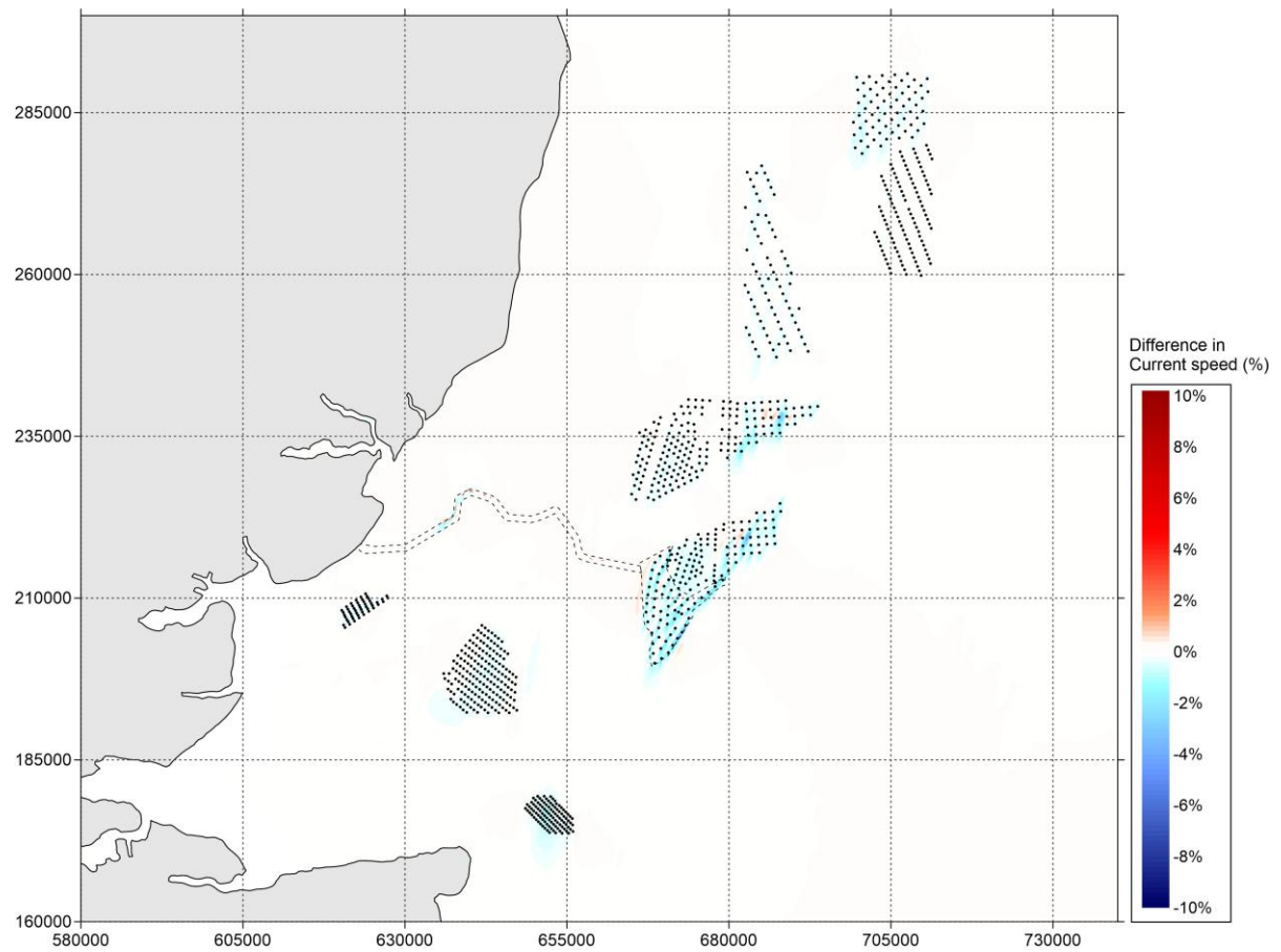
Figure 5-74 Difference in current speed (in percent) between 'Baseline' and 'Cumulative' during neap tide (positive means increase of current speed by option and vice versa) – peak flood
