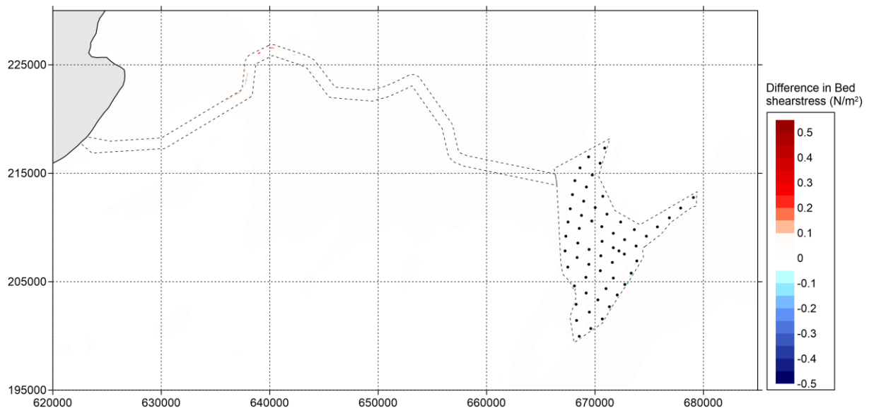
Figure 5-65 Difference in bed shear stress (in \text{N/m}^2 ) between 'Baseline' and 'Option' during neap tide (positive means increase of bed shear stress by option and vice versa) – peak ebb
