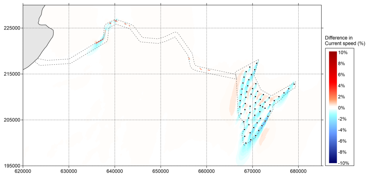
Figure 5-54 Difference in current speed (in percent) between 'Baseline' and 'Option' during spring tide (positive means increase of current speed by option and vice versa) – peak flood
