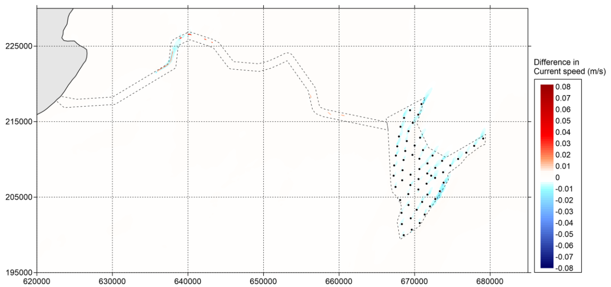
Figure 5-57 Difference in current speed (in metres/second) between 'Baseline' and 'Option' during neap tide (positive means increase of current speed by option and vice versa) – peak ebb
