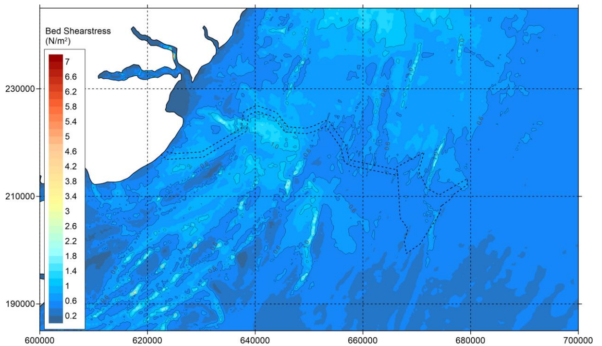
Figure 5-42 Baseline – Bed shear stress during neap tide - peak ebb (zoomed in).
