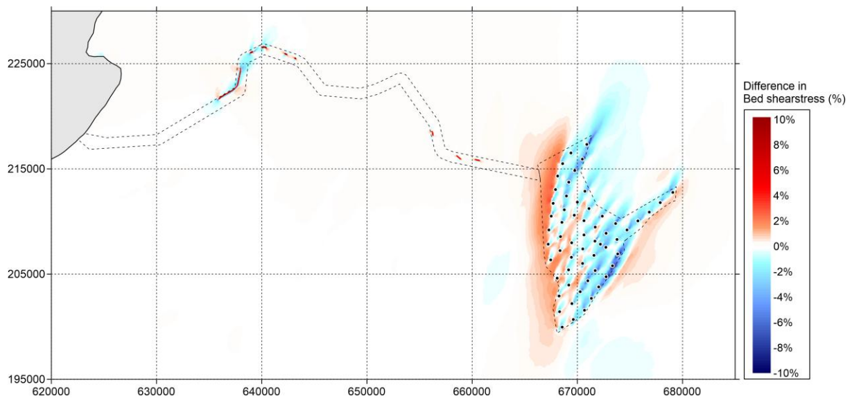
Figure 5-63 Difference in bed shear stress (in percent) between 'Baseline' and 'Option' during spring tide (positive means increase of bed shear stress by option and vice versa) – peak ebb
