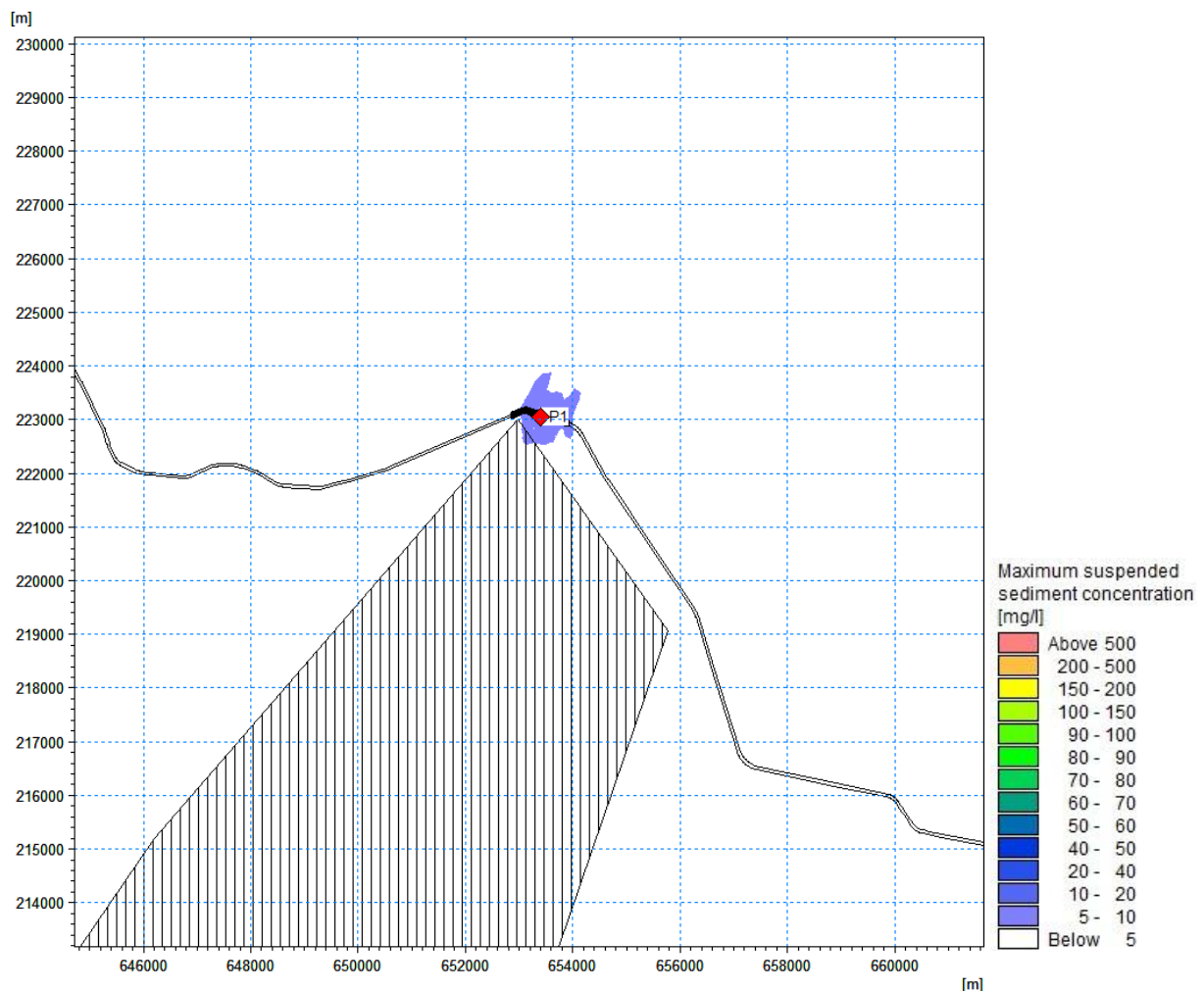
Figure 7-100 Maximum suspended sediment concentration during dredging operations at Pilot Boarding Area occurring near the seabed (red points = time series extraction point)
