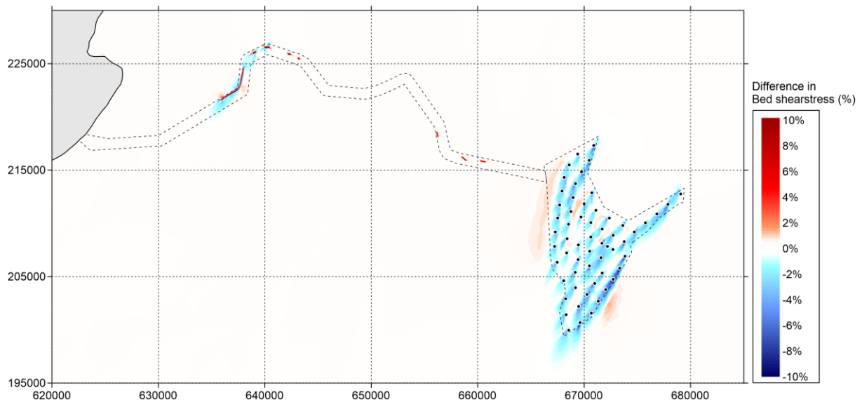
Figure 5-66 Difference in bed shear stress (in percent) between 'Baseline' and 'Option' during neap tide (positive means increase of bed shear stress by option and vice versa) – peak flood
