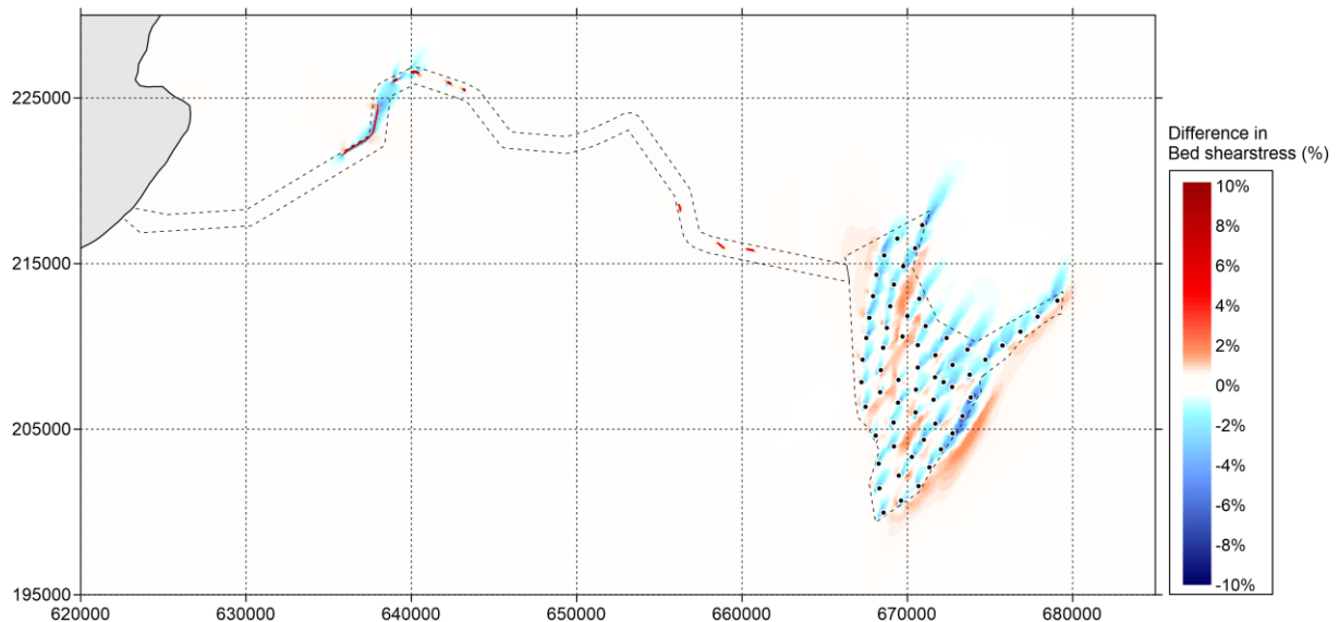
Figure 5-67 Difference in bed shear stress (in percent) between 'Baseline' and 'Option' during neap tide (positive means increase of bed shear stress by option and vice versa) – peak ebb
